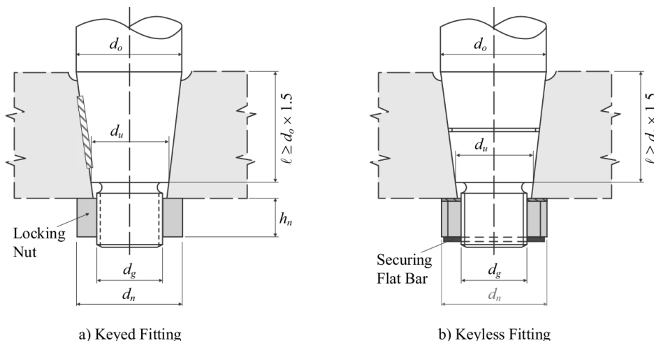
Fig. III 2-43 Tapered Couplings
