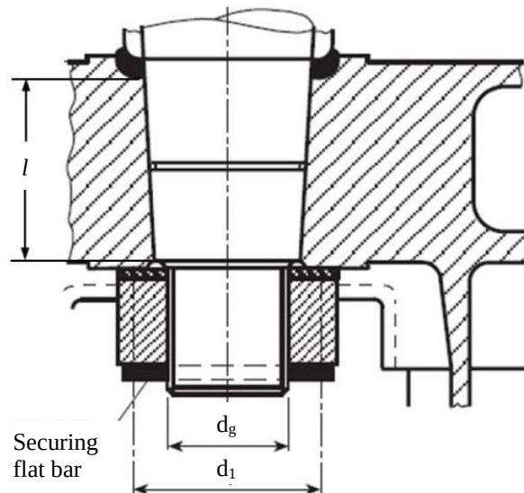
Fig. II 24-8 Cone Coupling without Key
