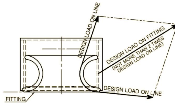
Fig. II 25-5 Design Load
