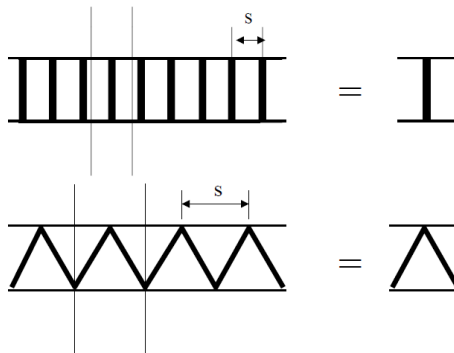
Fig. III 2-12 Extruded Planking
