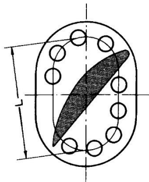
Fig. III 6-2 Blade Attaching Studs
